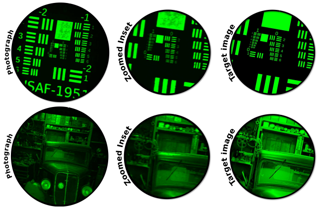
Figure 8: Captured photographs from the eyebox of our phase-only HoloBeam prototype. These photographs are captured using a XIMEA MC245MG-SY-UB image sensor equipped with an adjustable 5 – 50 mm lens while using 20ms exposure times. During these captures, only a green LED light source is used in the display prototype. The figure also shows zoomed-insets and their target images. The provided images are circular as the aperture of our eyepiece in this prototype is circular. The source image on the right side is from DIV2K [2].
