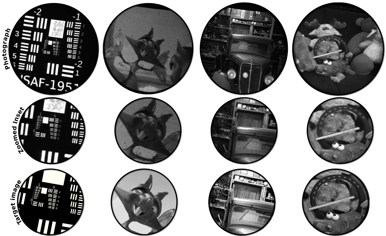
Figure 6: Resolution Quality of phase-only HoloBeam prototype. The first row shows captured photographs from the eyebox of our phase-only HoloBeam prototype. These photographs are captured using a XIMEA MC245MG-SY-UB image sensor equipped with an adjustable 5 – 50 mm lens while using 20ms exposure times to approximate a human observer’s view. During these captures, only a green LED light source is used in the display prototype. The second row shows zoomed-insets from the first row, while the third row shows the target images. The provided images are circular as the aperture of our eyepiece in this prototype is circular. The image quality of our phase-only HoloBeam approximates the ground truth images with a slight loss in contrast. The source image in the second, third and fourth column are from Big Buck Bunny [11], DIV2K [1] and Changil et al. [7], respectively.
