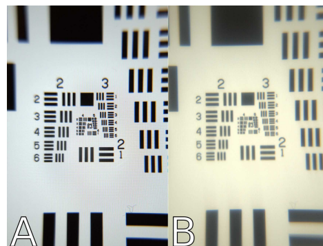
Fig. 8. Two photographs showing a view of a mobile phone display magnified by (Left) an off-the-shelf lens (Thorlabs LA1401), and (right) a clone of the same lens manufactured using our technique, to provide a visual comparison of optical quality.
