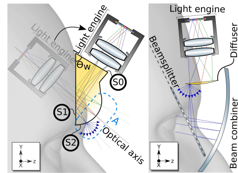
Fig. 3. There are two options for optical path folding in our proposal. Sketches show (Left) an optical waveguide design merged with our freeform projection surfaces, (right) traditional birdbath optics with beam splitters.
