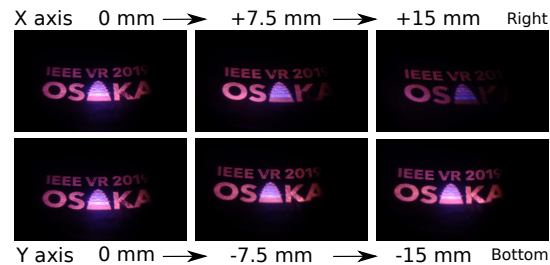
Fig. 11. Evaluating the eyebow properties of our benchtop prototype with a series of photographs taken from different locations inside the eyebow. The two rows show the view as seen through the corresponding viewpoint location in the benchtop prototype. The top row demonstrates the eyebow properties along the X axis relative to the center point and the bottom row shows eyebow properties along Y axis relative to center.
