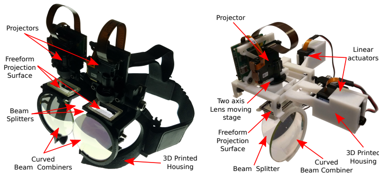
Fig. 9. Two photographs showing our Near-Eye Displays that use interchangeable freeform projection surfaces with birdbath optics. The photograph on the left shows our untethered wearable Near-Eye Display prototype, and the photograph on the right shows our bench-top prototype with projection lens steering capabilities.
