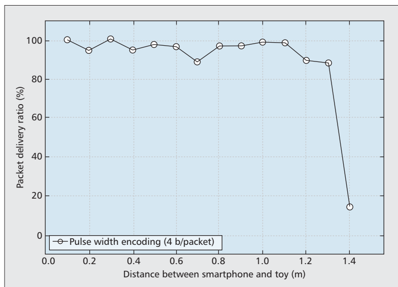
Figure 4. Smartphone-to-LED communication mode: packet delivery ratio over distance for a flashlight communicating to a toy; throughput: up to 2 b/s. Results are shown for distances of up to 1.5 m. The flashlight speed limits the throughput.
