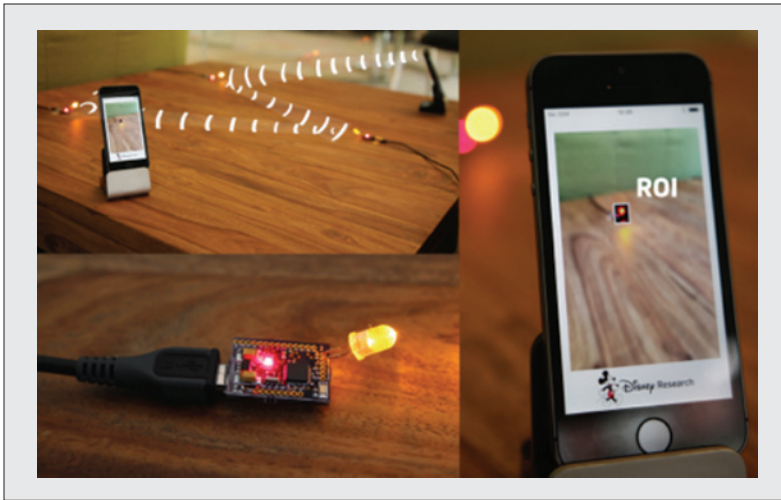
Figure 2. Photographs showing different parts of the integrated system: top left: a view of the overall experimental setup from the top; bottom left: a microcontroller with an LED able to act as a transceiver; right: a smartphone running an application developed for experimental tests.
