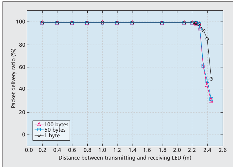
Figure 3. LED-to-LED communication mode: packet delivery ratio over distance for two communicating LEDs; throughput: up to 8 kb/s. Results are shown for distances of up to 2.5 m and for packet sizes of 1, 50, and 100 bytes. The communication protocol described in [7] is used for the data exchange.
