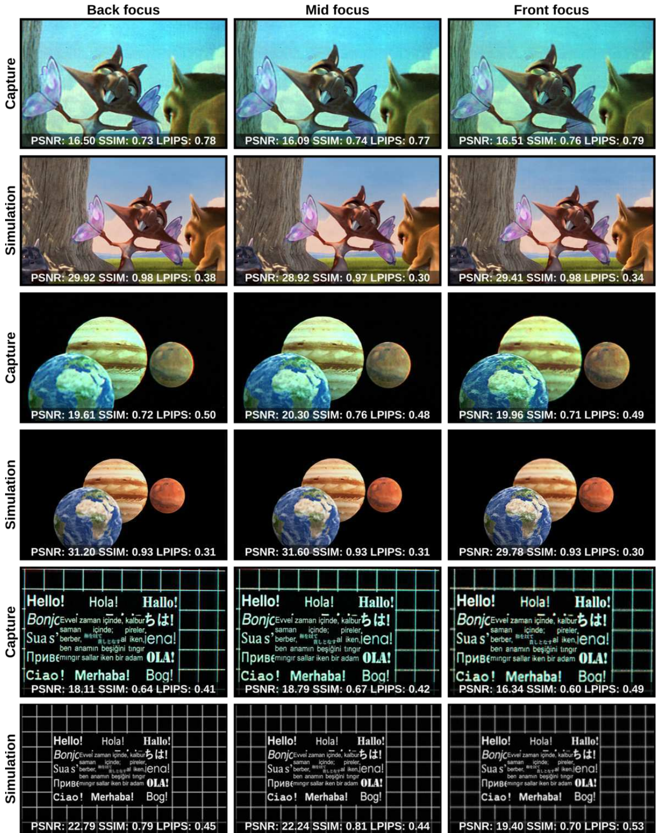
Figure 3: Additional capture and simulation results of our method with various different scenes and focuses. The provided captures are generated on the Spatial Light Modulator (SLM) plane. All the images are captured with 20 ms exposure time using our holographic display. The provided simulated images are also generated on the Spatial Light Modulator (SLM) plane. All the simulated images are results from our hologram reconstruction simulation using our method. Both in captures and simulations, there are six target image planes in depth with 1 mm separation between each depth plane (-2.5 mm and +2.5 mm with respect to an SLM).
